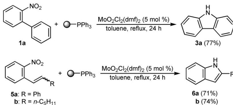
Scheme 2. Dioxomolybdenum-catalyzed reductive cyclization of 2-nitrobiphenyl 1a and 2-nitrostyrenes 5a and b with polymer-bound PPh 3 .
