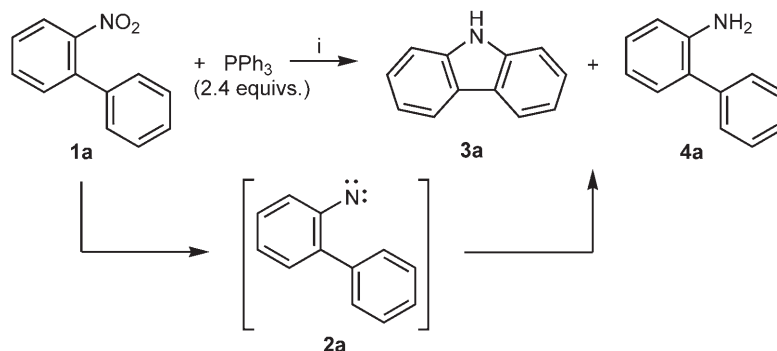
Scheme 1. Optimization of the reductive cyclization of 2-nitrobiphenyl 1a to carbazole 3a . Reagents and conditions: i) MoO 2 Cl 2 (dmf) 2 (5 mol %), solvent, reflux, time (see Table 1).
