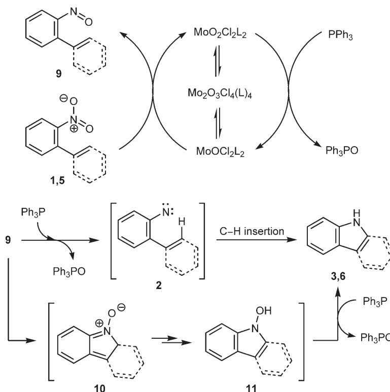
Scheme 3. Proposed mechanisms for the reductive cyclization of nitroaromatics 1 and 5 .
